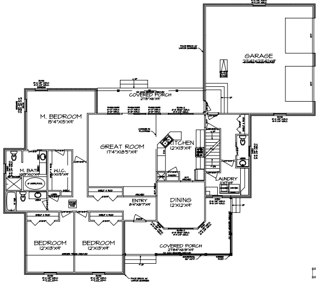
1 FIRST FLOOR PLAN A-4 SCALE: 1/4"=1'-0"
