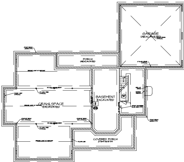
1 FOUNDATION PLAN A-3 SCALE: 1/4"=1'-0"
